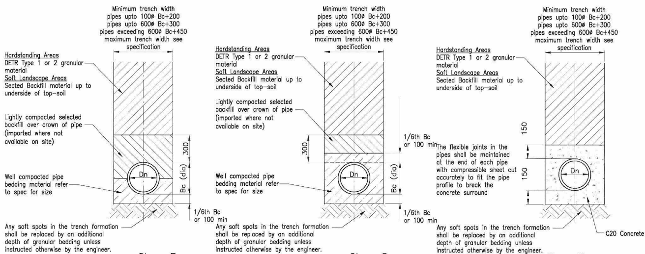
Class B 180° Granular Bed Pipe Bedding Detail
