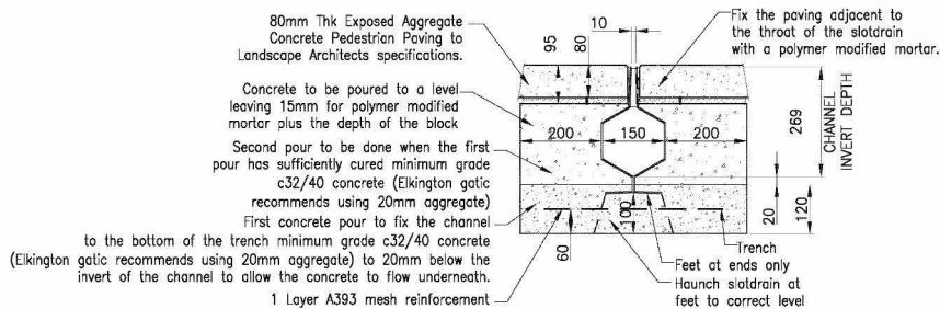
SLOT DRAIN DETAIL
