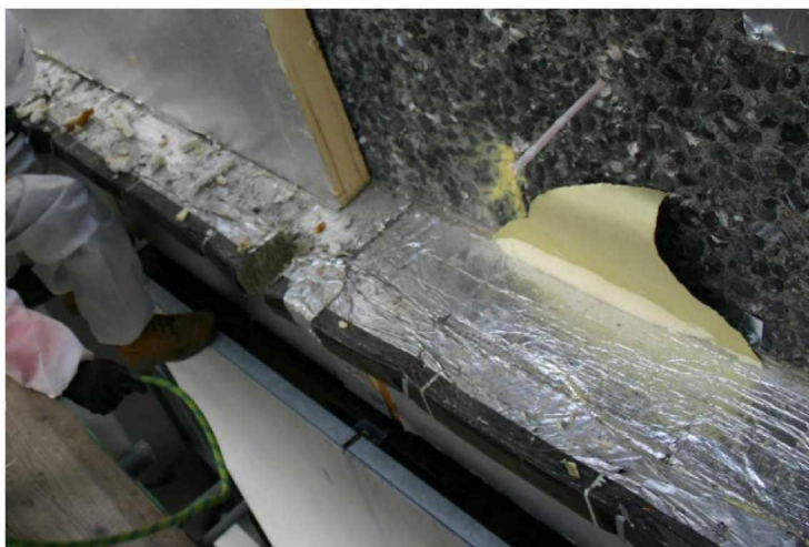
(b) Horizontal cavity barrier affixed to spandrel – upside down position indicated by absence of green logo on top surface
