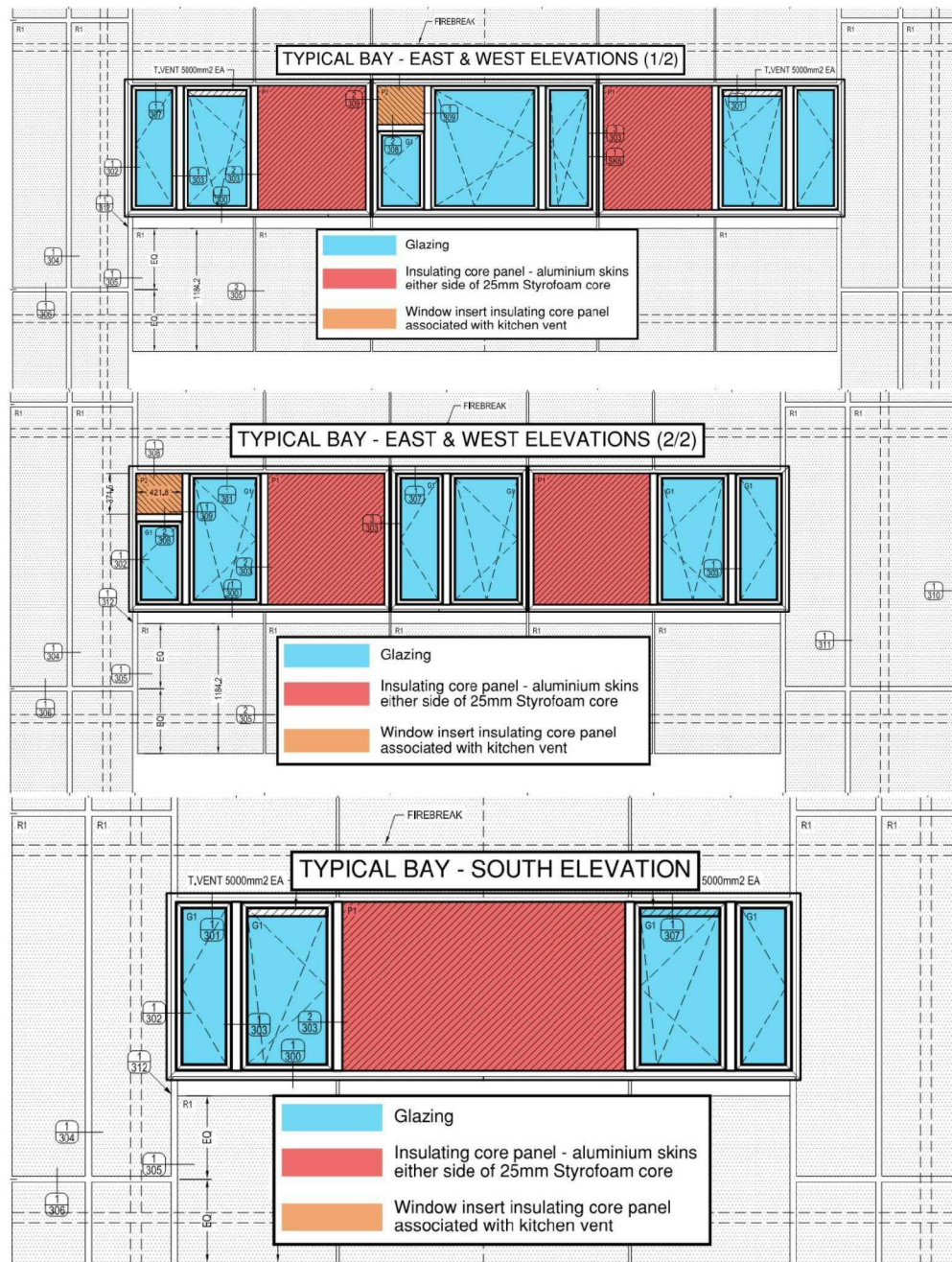
Figure 11.8 Location of insulating core panel and the type of insulation (Adapted from construction drawings C1059-200 Rev I [HAR00008581], C1059-201 Rev D [HAR00008582], C1059-202 Rev C [HAR00008583])
