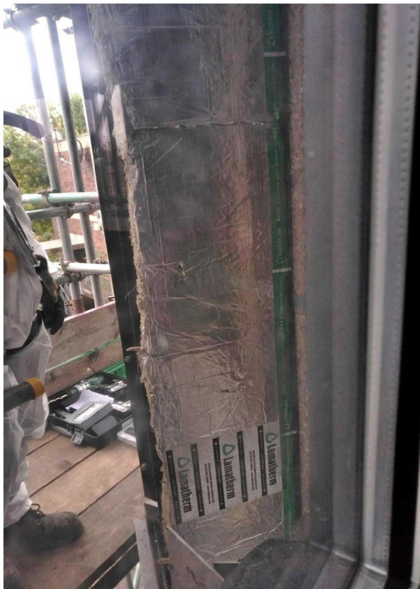
Figure 11.30 Siderise RH horizontal application cavity barrier installed vertically, with intumescent strip facing column D1 outside flat 13 (indicated by green Siderise RH logo)
