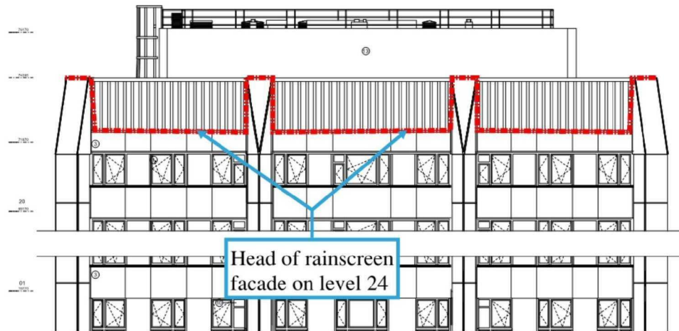
Figure 11.32 Location of the head of the rainscreen cladding at level 24 (adapted from drawing 1265 PL 322 Rev 03, RYD00092648)
