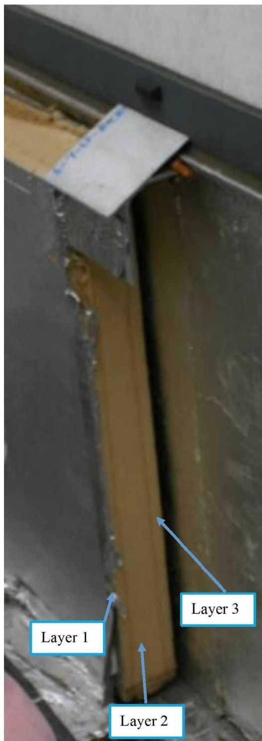
Figure11.16 Celotex on spandrels observed to be formed of three layers
