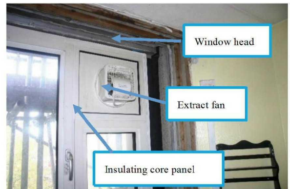
(b) Non-glazed insulating core panel in place (flat 13 on level 4)
