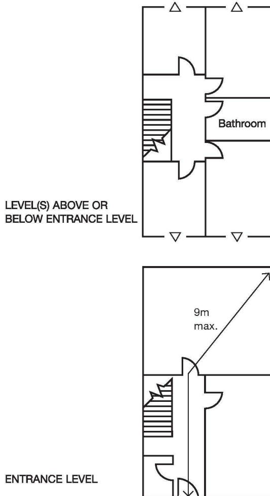
Diagram 5 Multi-storey flat with alternative exits from each habitable room, except at entrance level
