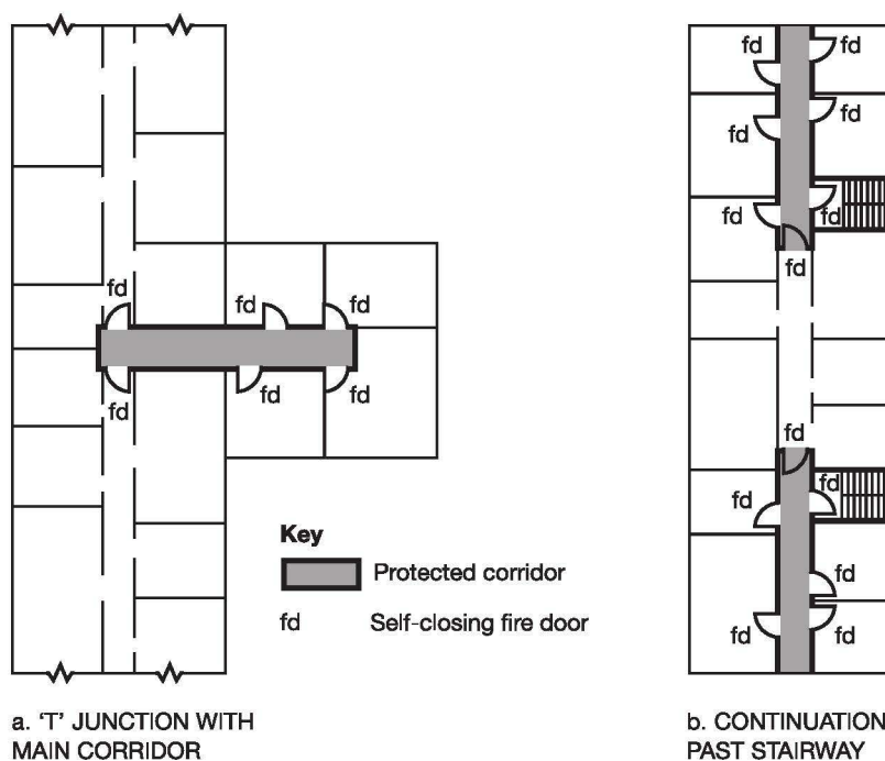
Diagram 17 Dead-end corridors
