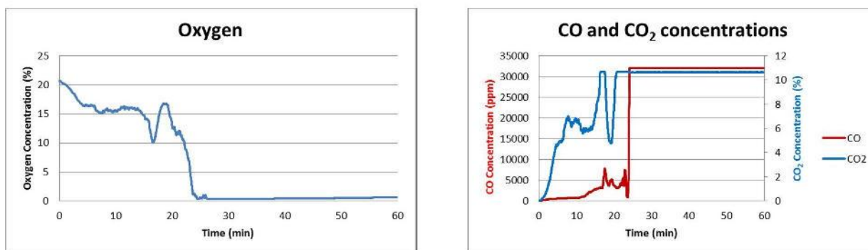
Figure 13 – Gas concentrations (by volume) for Experiment 5
