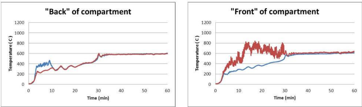
Figure 15 - Temperatures at the front (B3) and back (B2) of the experimental rig for Experiment 6
