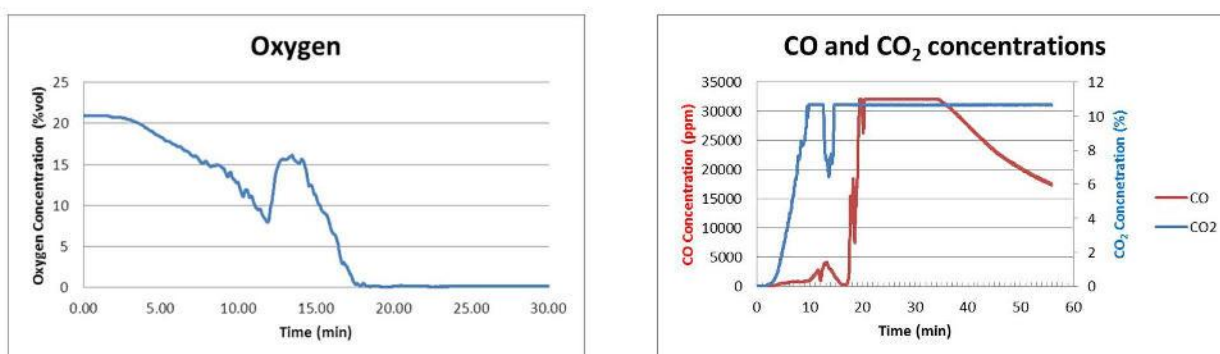
Figure 10 – Gas concentrations (by volume) for Experiment 4
