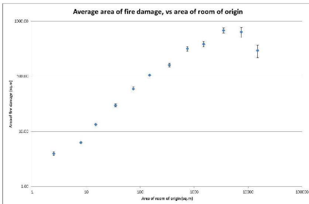
Figure 1 – Graph of average area of fire damage ( \text{m}^2 ) versus area of room of fire origin ( \text{m}^2 ) (sample size 263,000 fires)
