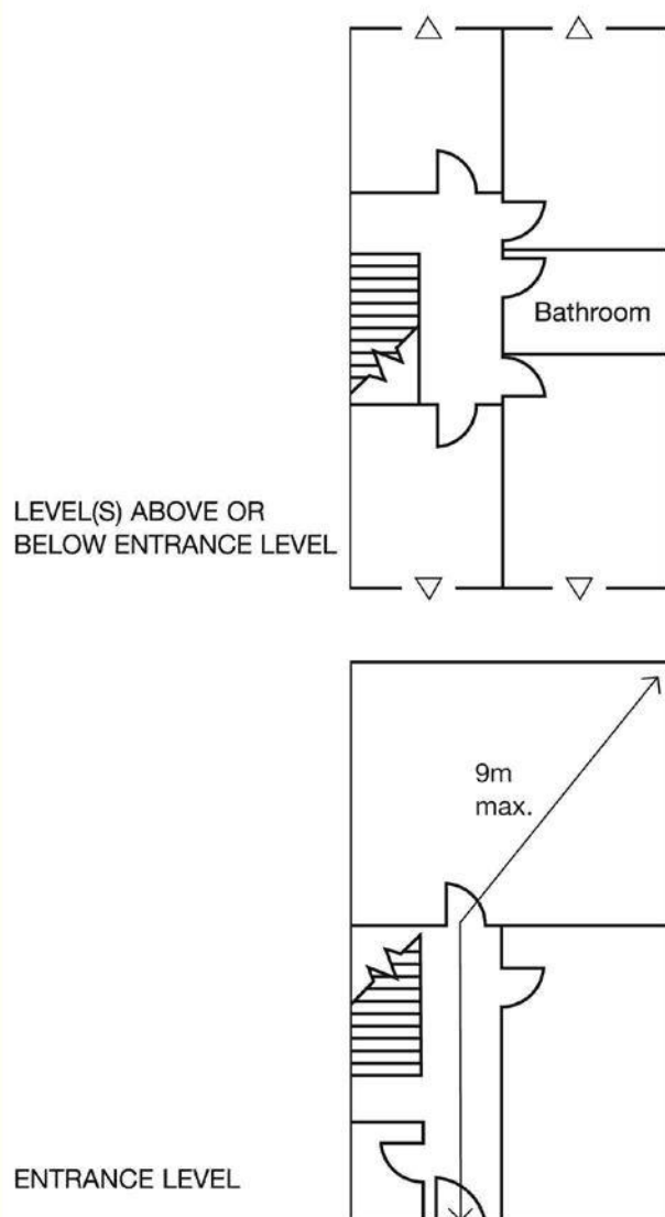
Figure 6 – Multi storey flat with alternative exits, from each habitable room, except at entrance level
