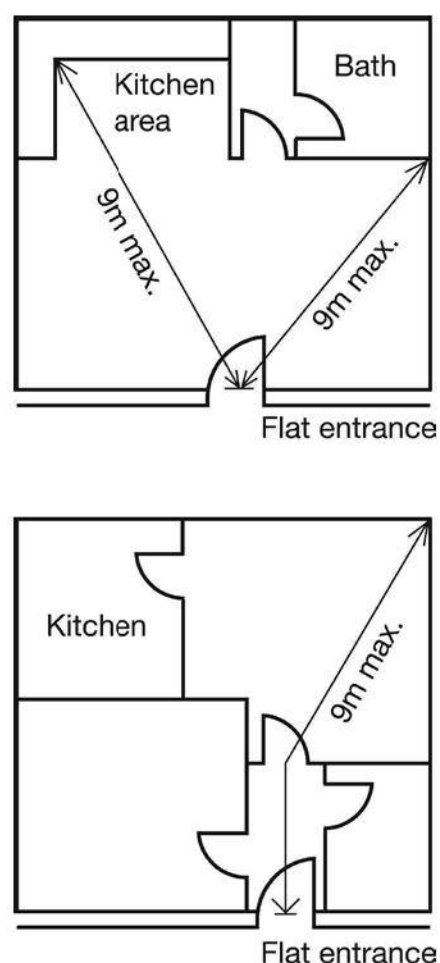
Figure 3 – Flat with limited travel distance
