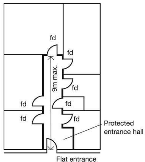
Figure 4 – Flat with a protected entrance hall
