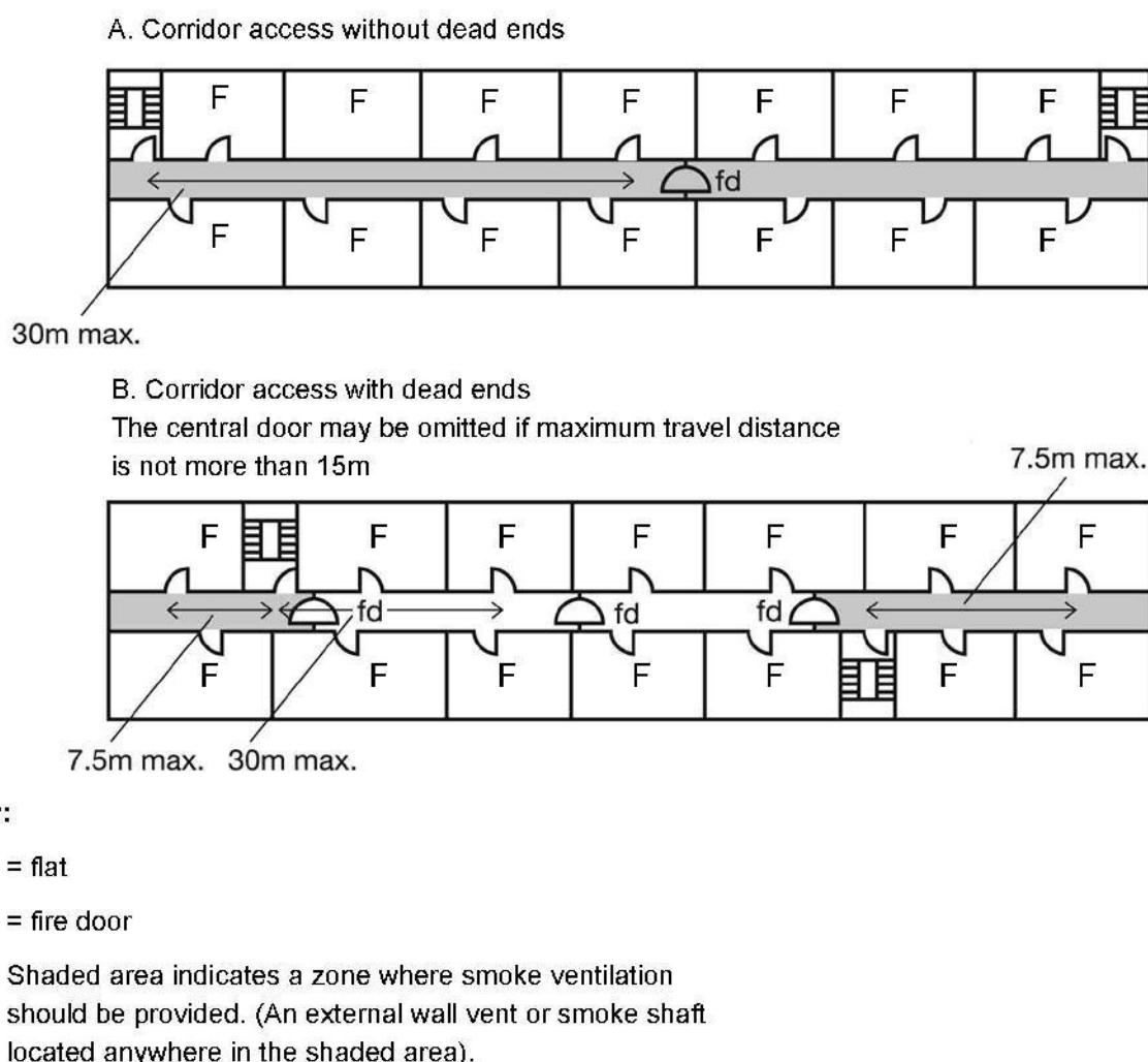
Figure 9 – Flats served by more than one escape stairway
