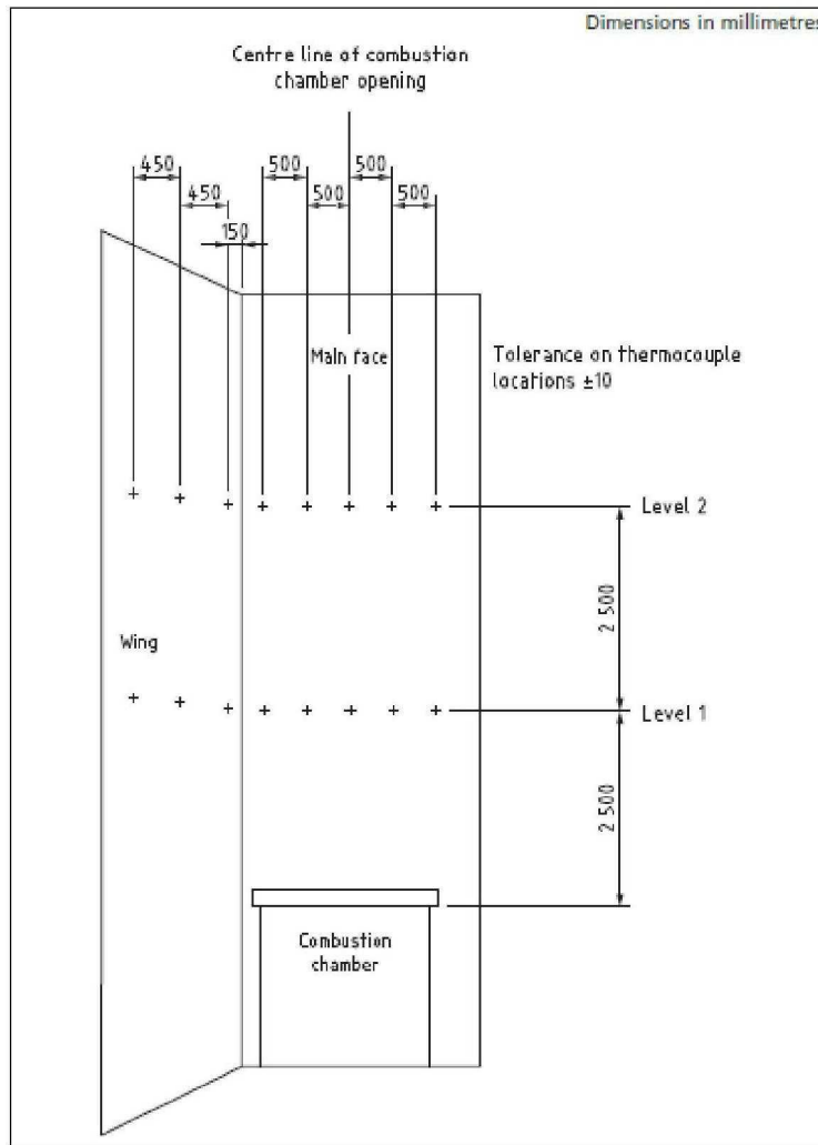
Figure 1: BS 8414 Test Rig (Reproduced from BS 8414-1)
