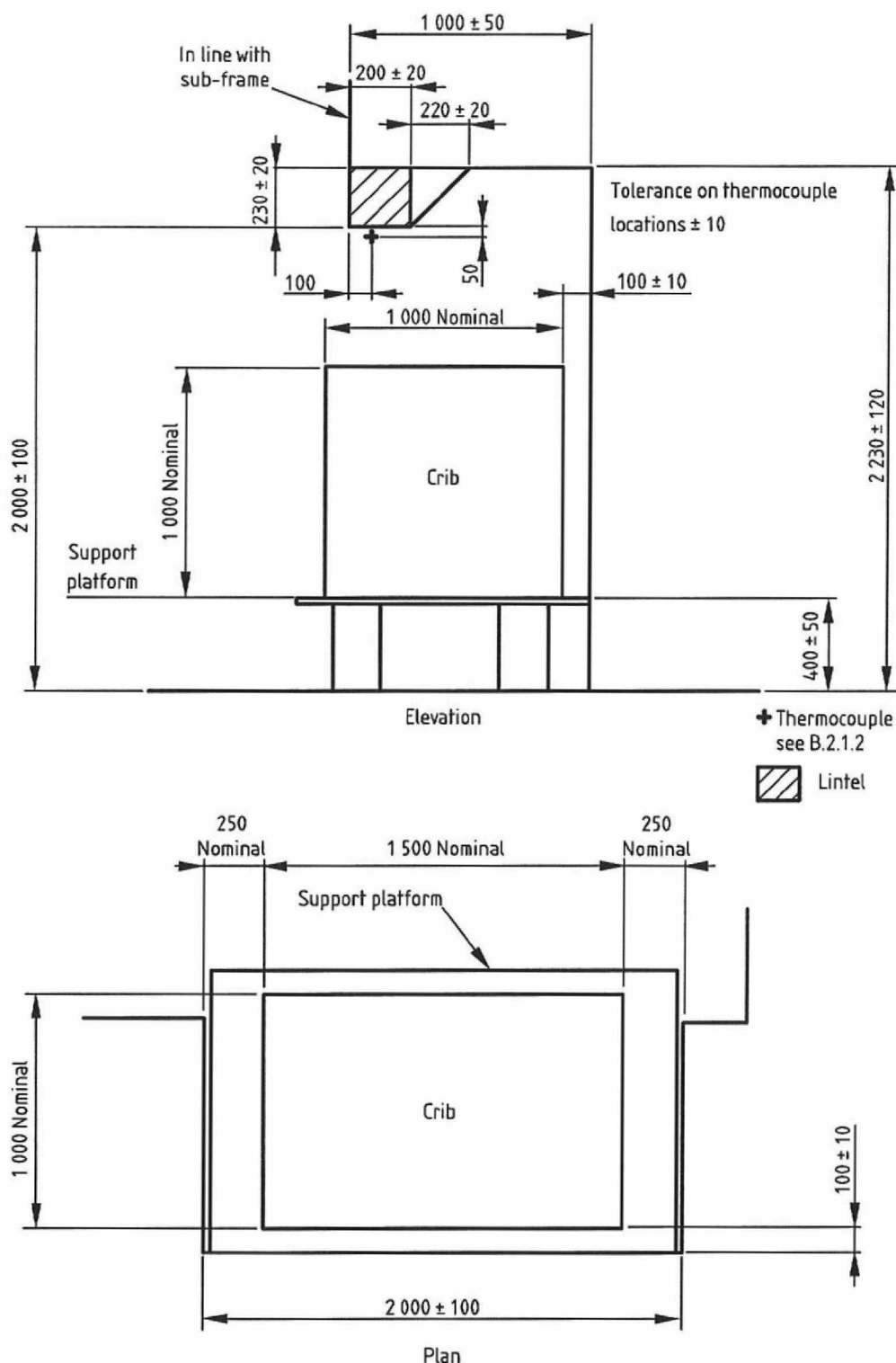
Figure C.1 — Elevation and plan of the combustion chamber
