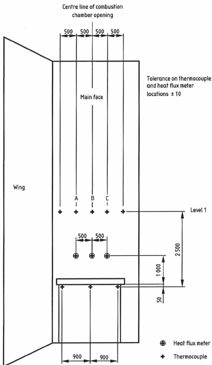
Figure B.1 — Location of heat flux meters and thermocouples for calibration test
