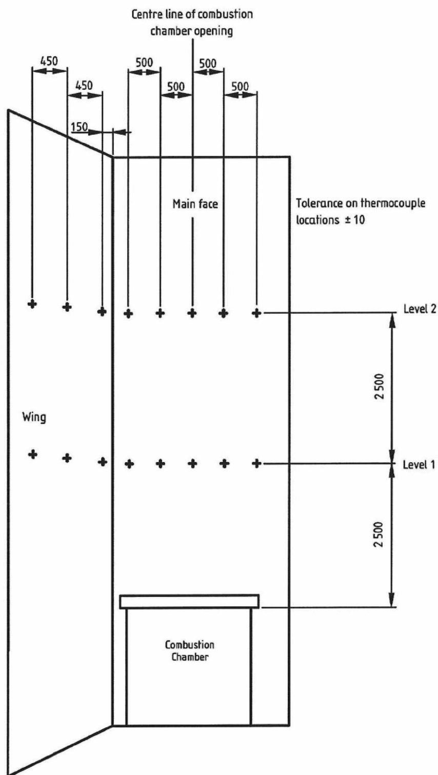
Figure 2 — Location of thermocouples for a cladding test
