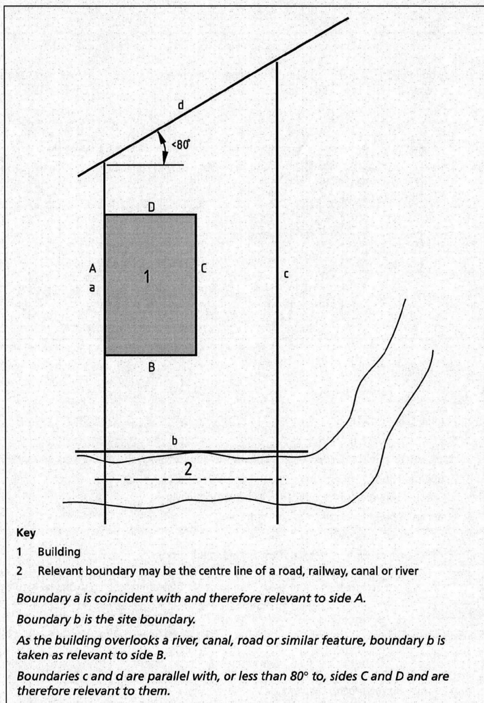
Figure 20 Relevant boundaries
