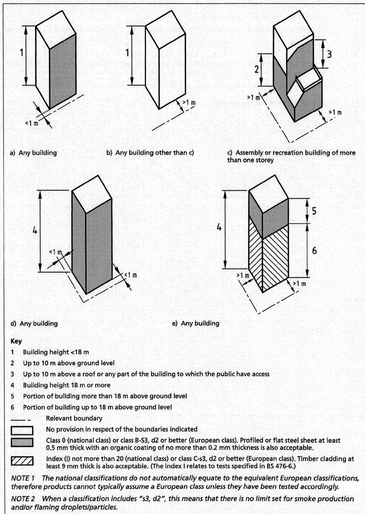
Figure 19 Provisions for external surfaces of walls
