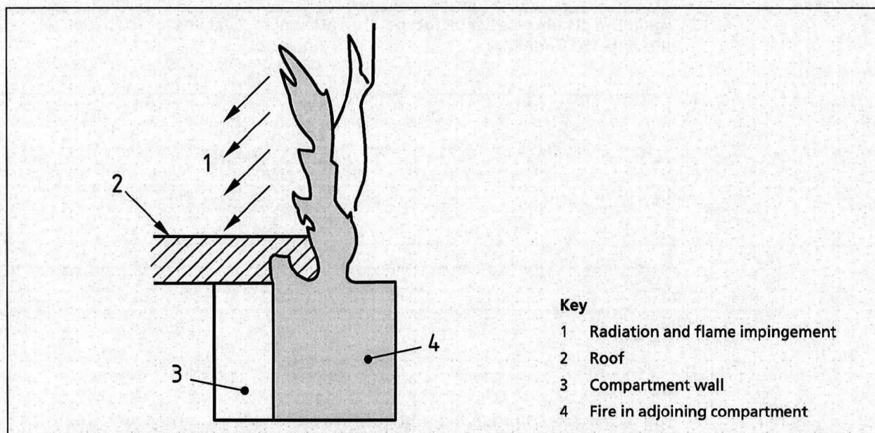
Figure 24 Roof covering adjoining line of compartmentation
