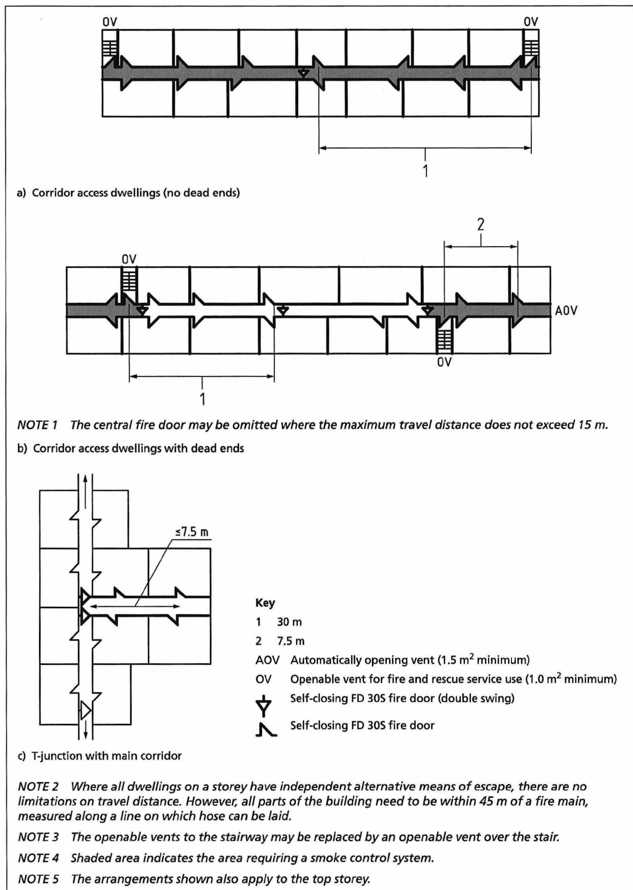
Figure 7 Common escape routes in multi-stair buildings
