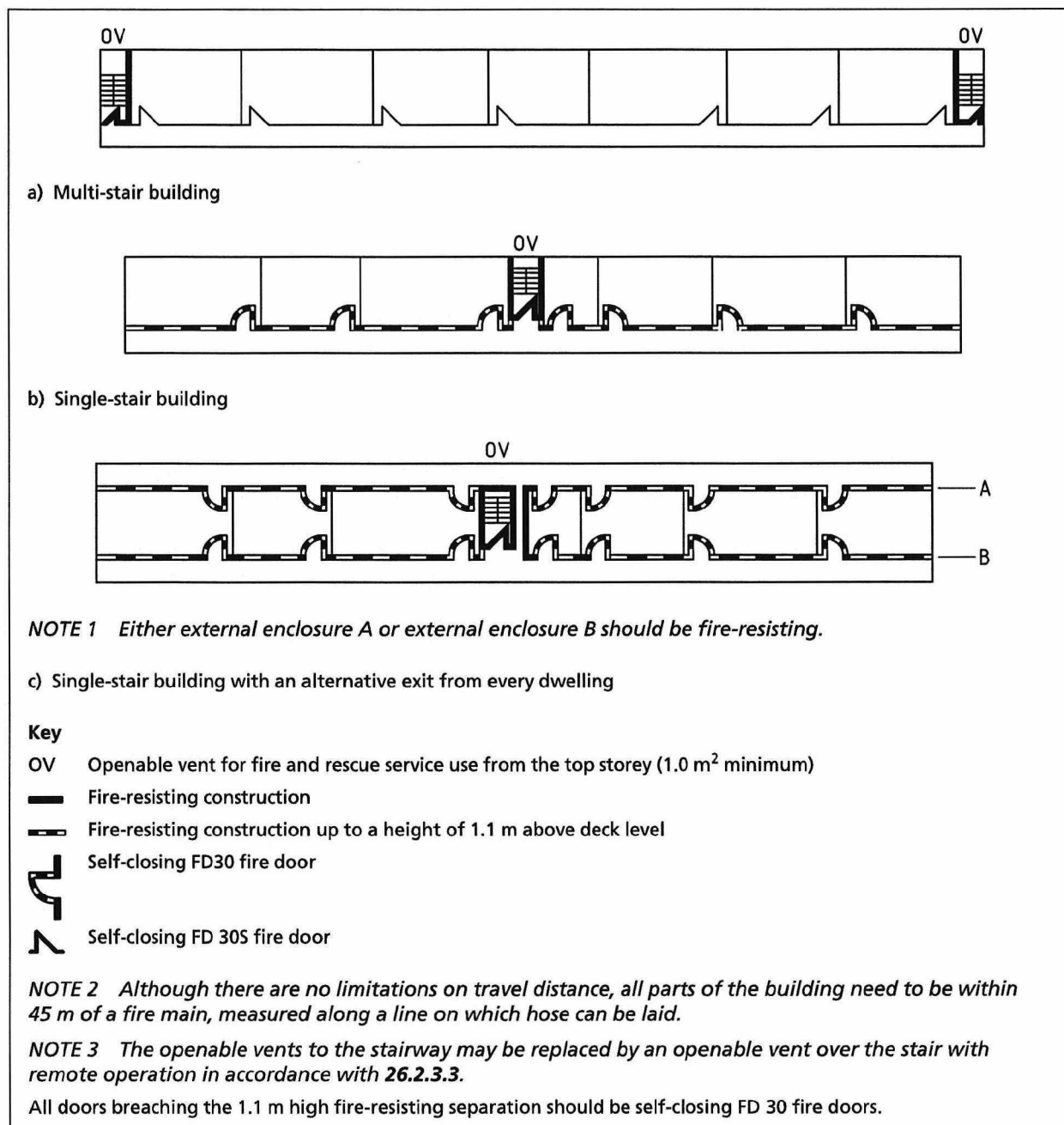
Figure 5 Common escape routes in balcony/deck approach buildings
