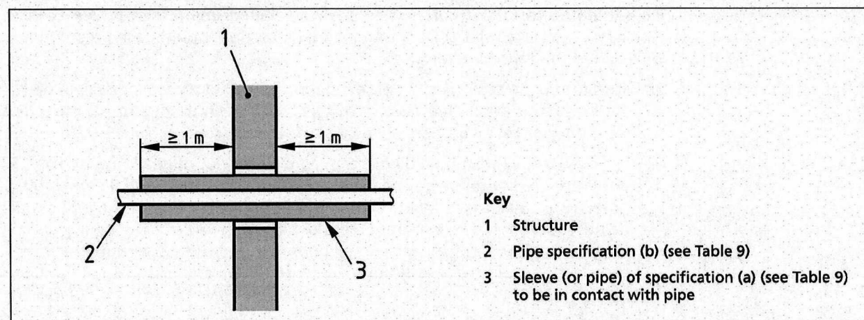
Figure 32 Pipes penetrating structure
