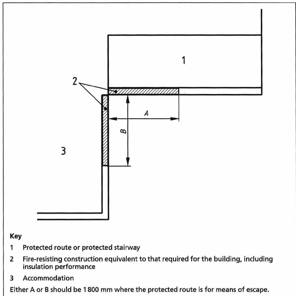
Figure 16 Protected routes forming an internal angle
