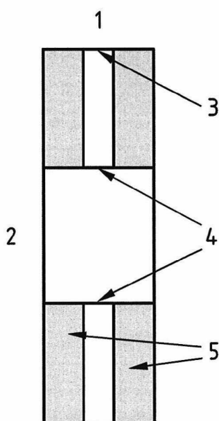
Figure 27 Cavity wall excluded from provisions for cavity barriers
