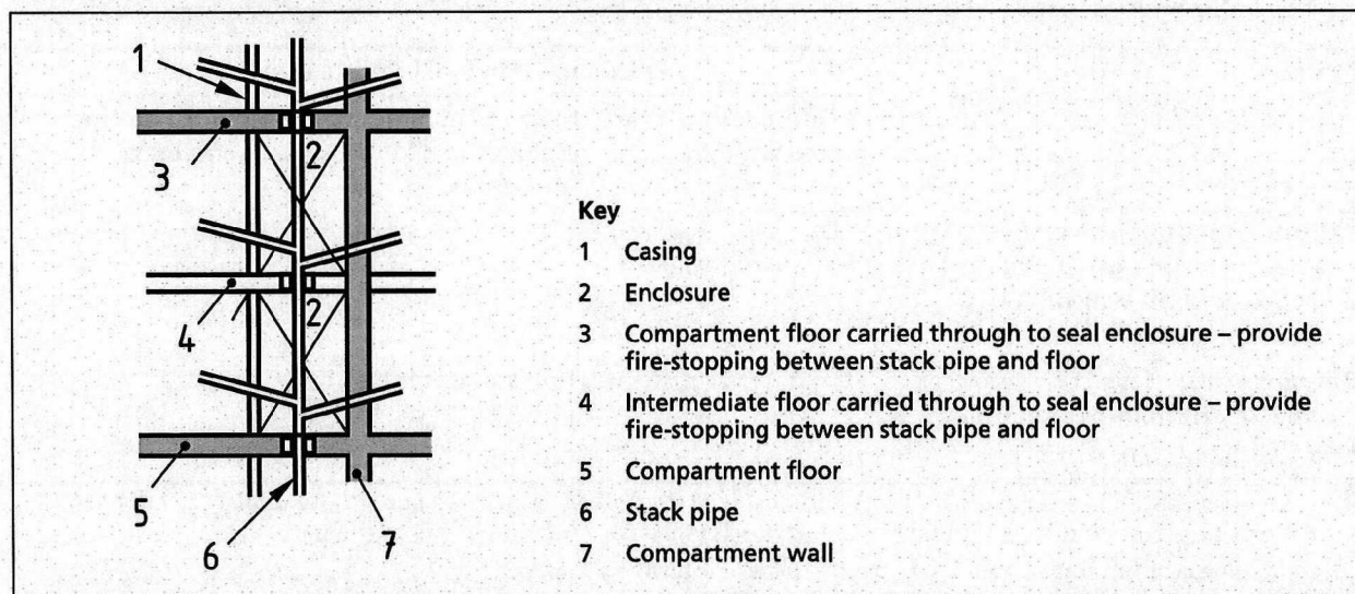
Figure 31 Enclosure for drainage or water supply pipes
