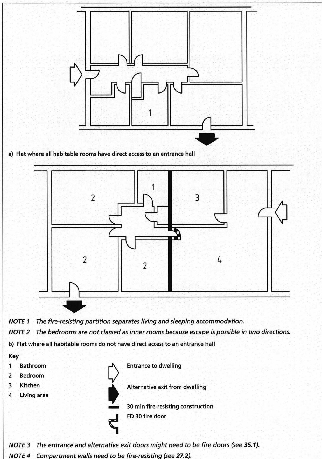
Figure 12 Flat with an alternative exit
