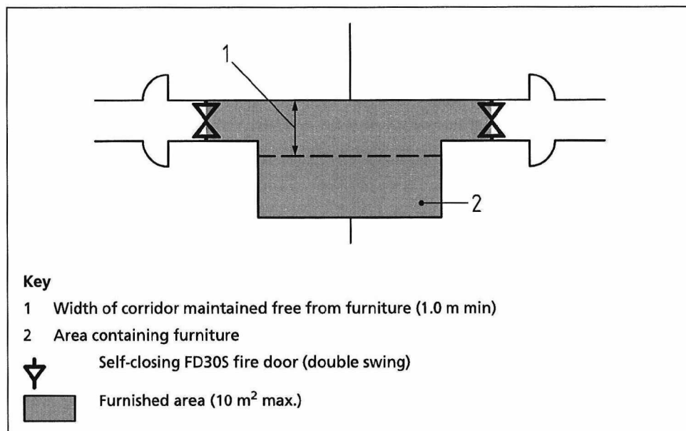
Figure 9 Furnished areas in sheltered housing corridors
