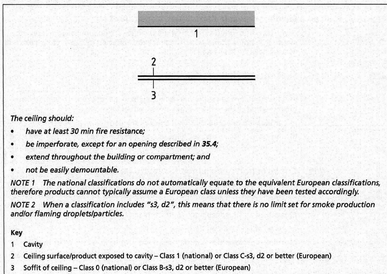
Figure 28 Fire-resisting ceiling below concealed space
