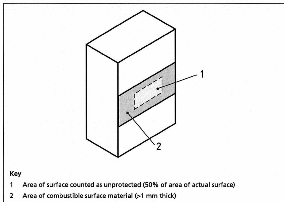
Figure 22 Combustible surface material as unprotected area
