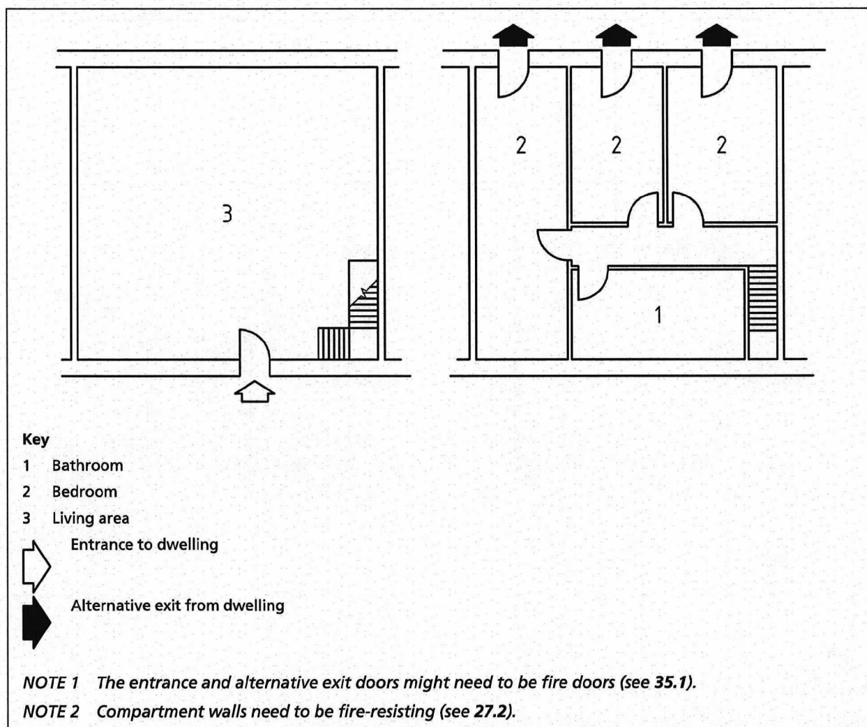
Figure 4 Open-plan maisonette
