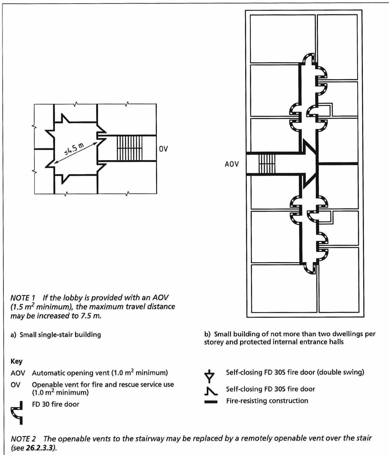
Figure 8 Common escape routes in small single-stair buildings
