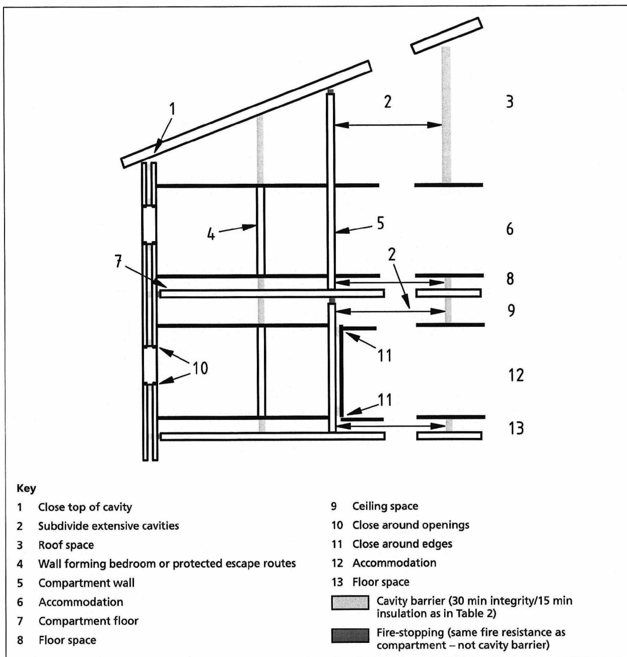
Figure 26 Provisions for cavity barriers
