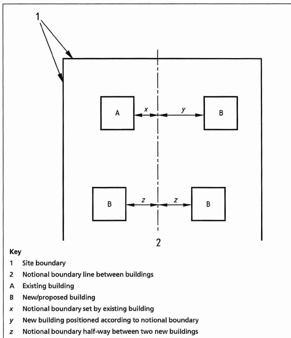
Figure 21 Notional boundaries
