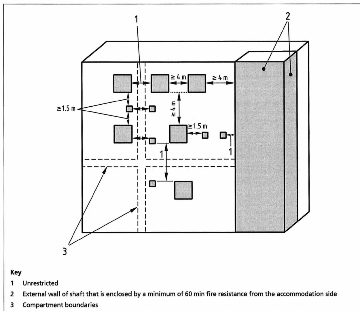
Figure 23 Exclusions from unprotected area calculations
