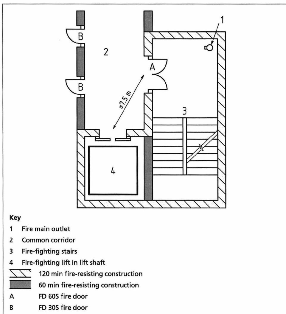
Figure 18 Components of a residential fire-fighting shaft
