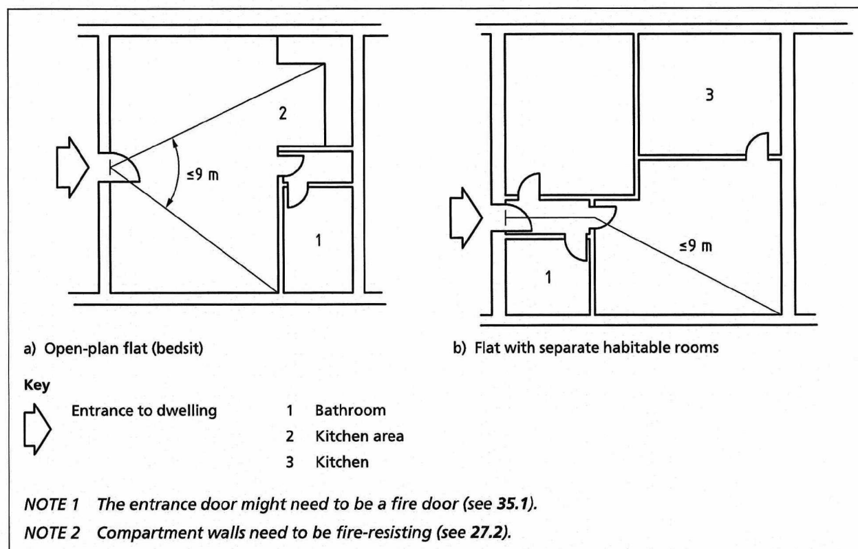
Figure 10 Flat with restricted travel distance
