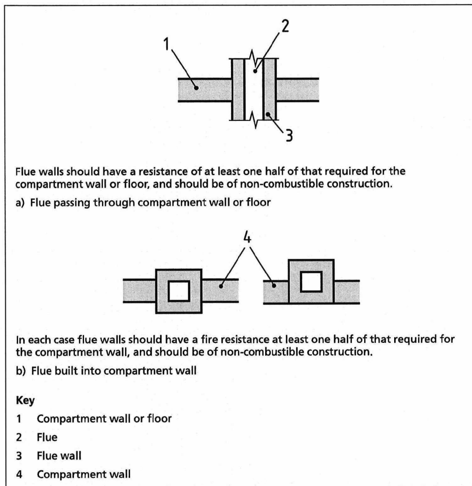
Figure 30 Flues and compartment walls and floors
