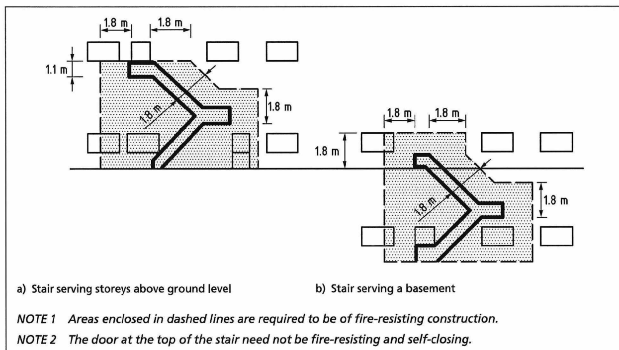
Figure 17 Fire resistance of areas adjacent to external stairs
