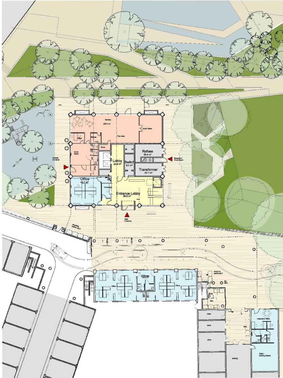
GROUND FLOOR
