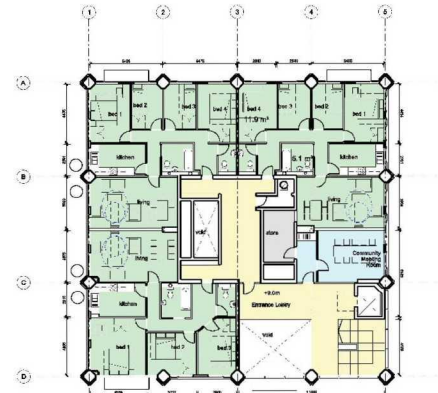
MEZZANINE LEVEL
