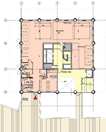
WALKWAY LEVEL
