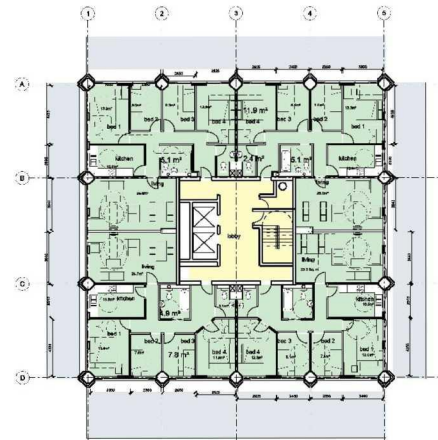
OFFICE LEVEL
