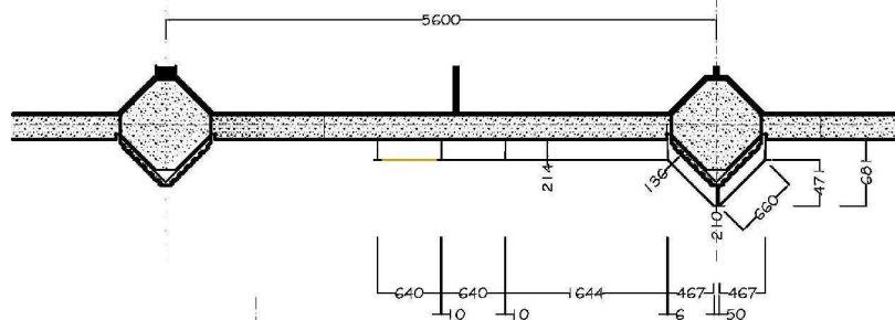
Enlarged Plan View. Scale- 1:20
