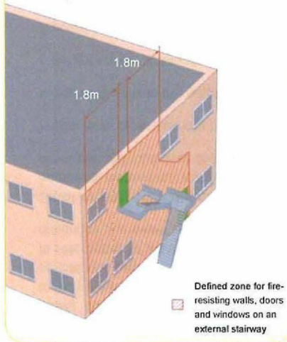
Figure 11 – Protection to an external stairway
