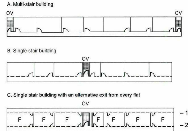
Figure 10 – Common escape routes in balcony/deck approach blocks
