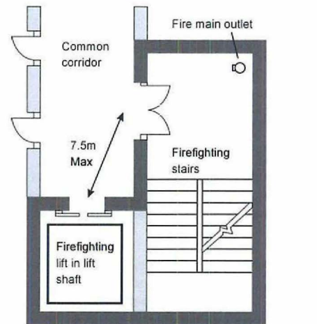
Figure 13 – Basic components of a fire-fighting shaft
