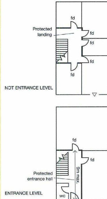
Figure 7 – Multi-storey flat with protected entrance hall and landing
