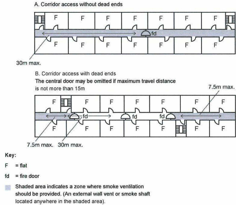
Figure 9 – Flats served by more than one escape stairway
