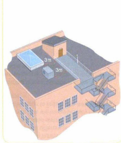
Figure 12 – Escape route across a roof
