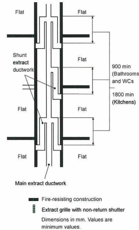
Figure 1 – Shunt duct arrangements
