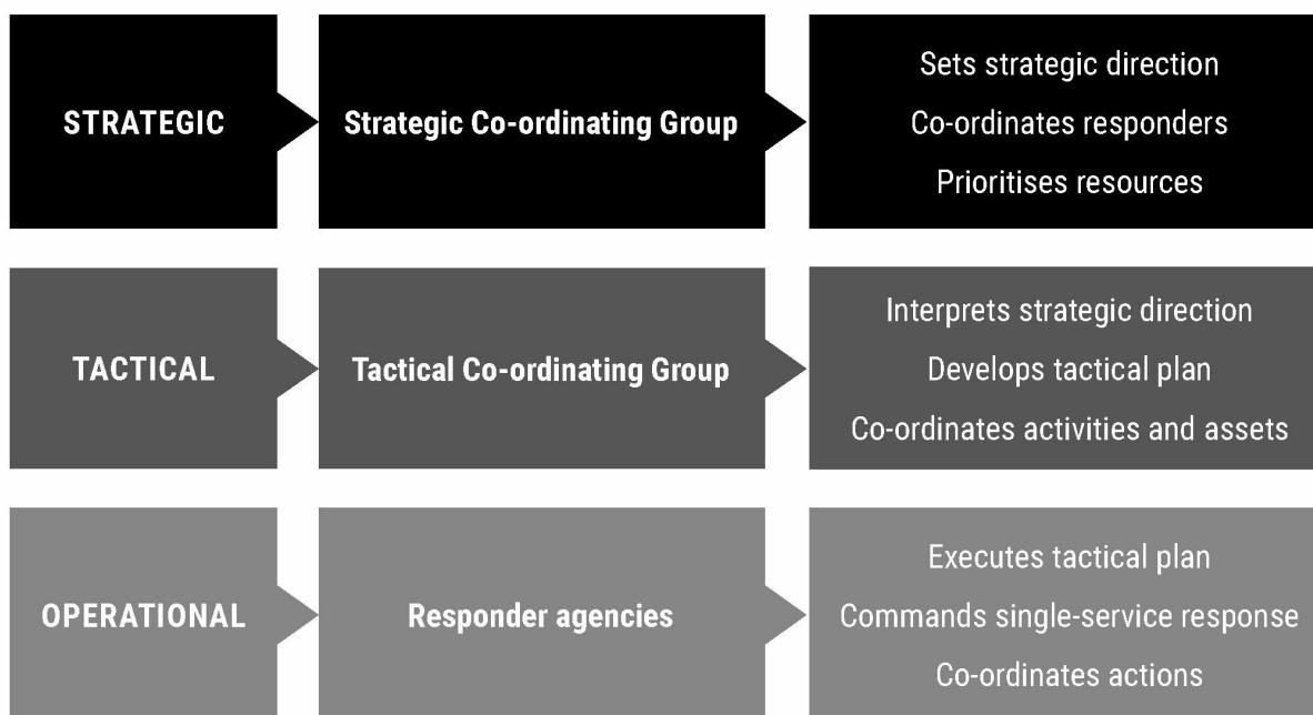
Figure 4 - Response structure
