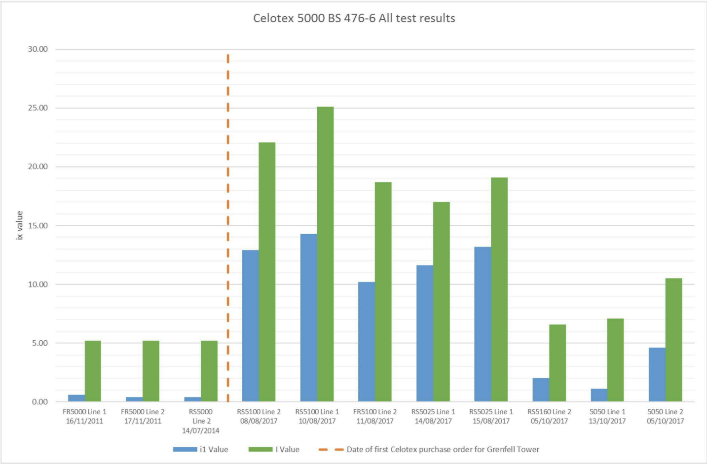
Figure E1 Celotex 5000 BS 476-6 test results
