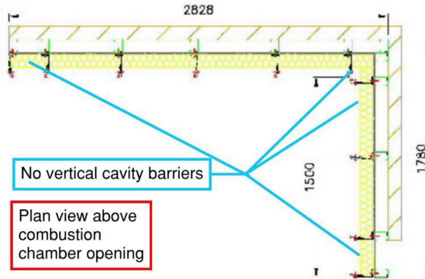
Figure E.6 BRE report figure 7 (CEL00000374) no vertical cavity barriers shown however test photo shows them in place
