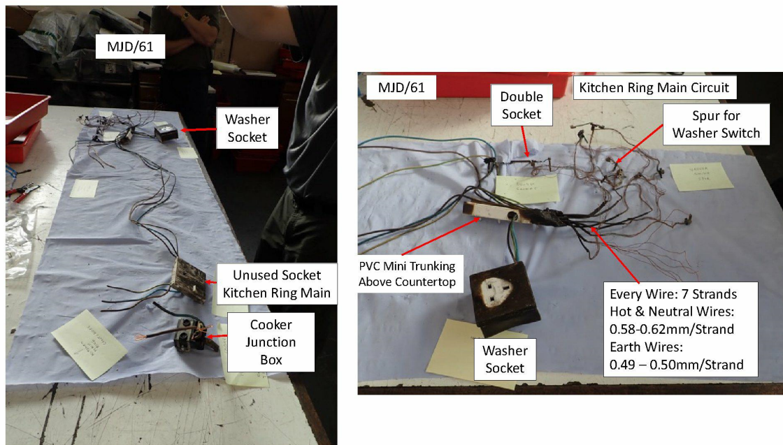
Figure A12-3: MJD/61: Wiring from Wall to Left of Sink [J.D. Glover Photo – 21 September 2018]
