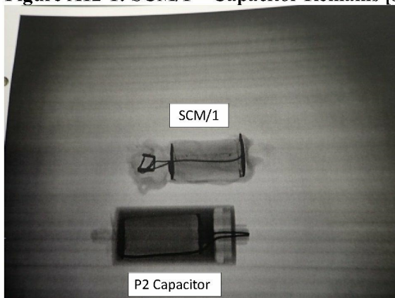
Figure A12-1: SCM/1 – Capacitor Remains [J.D. Glover Photo – 26 September 2018]
