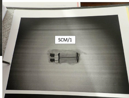
Figure A12-2: X-Rays of SCM/1 and P2 Capacitor [J.D. Glover Photo – 21 September 2018]
