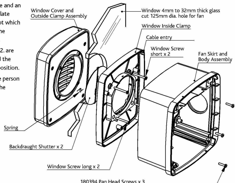
Fig 3. Kit components.
