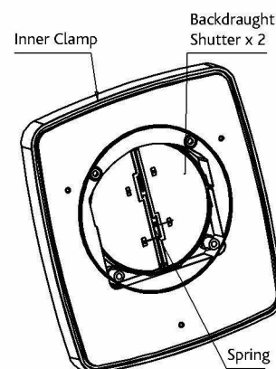
Fig 2. Spring assembly.
